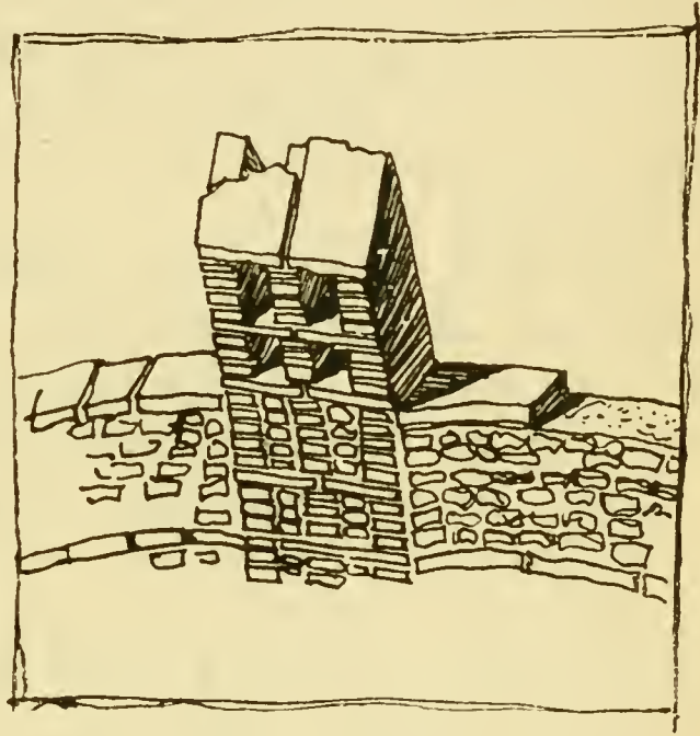
FIG. 60. Ribs in the cupola of the so-called Temple of Minerva Medica at Rome.
